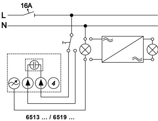
Afb. 3: Dimmer in wisselschakeling
