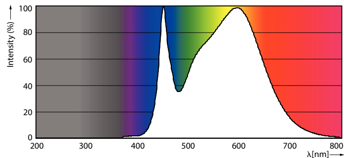
Spectral Power Distribution Colour - MAS LEDtube HF 600mm HO 8W840 T8
