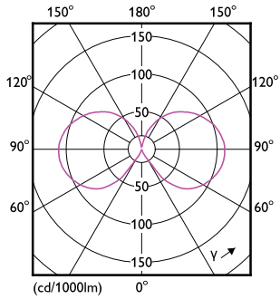
Light Distribution Diagram - CorePro LEDCandleND2.2-25W E14 840B35CLG
