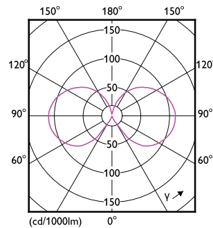
Light Distribution Diagram - CorePro LEDLusterND2.2-25W E14 840P45CLG
