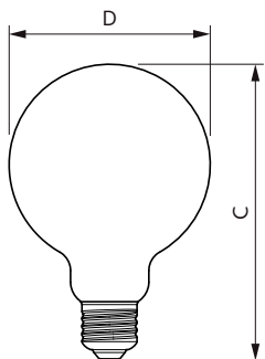
MASTER VLE LEDBulb DT5.9-60W E27 927G93CL G
