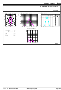
Accent Lighting Spots - MAS LED spot VLE D 2.8-35W GU10 927 36D
